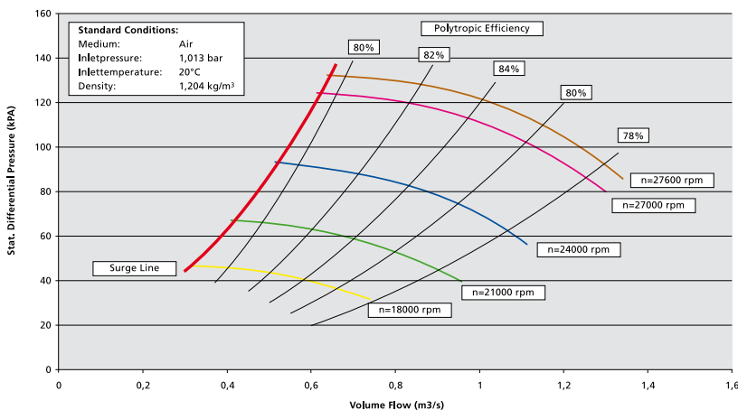
Performance Curve 5069 MTC 50125
